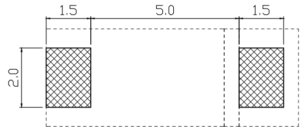
PCB Weld zone
